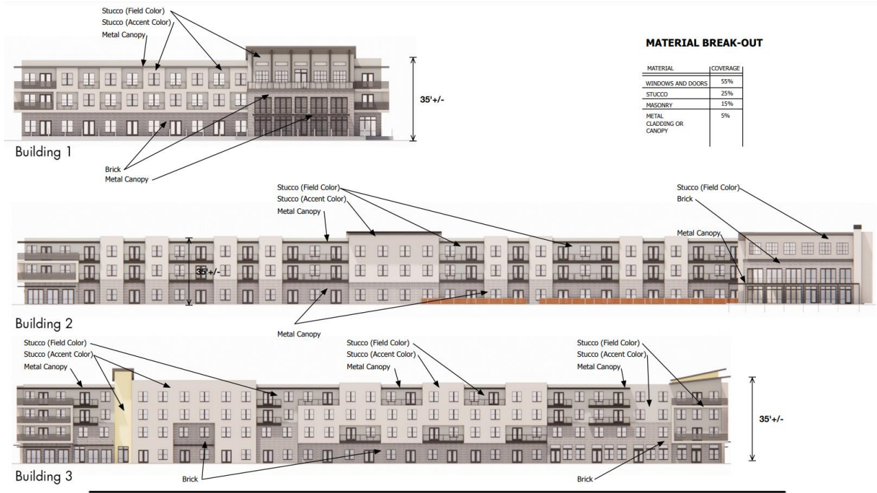
BUILDING ELEVATIONS WITH MATERIAL CALL-OUTS
