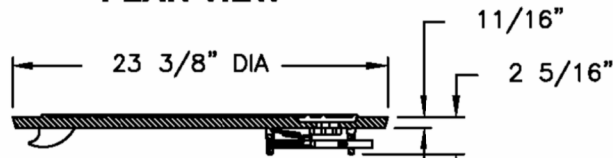
COVER SECTION
