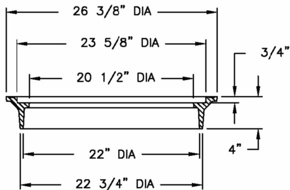
FRAME SECTION
